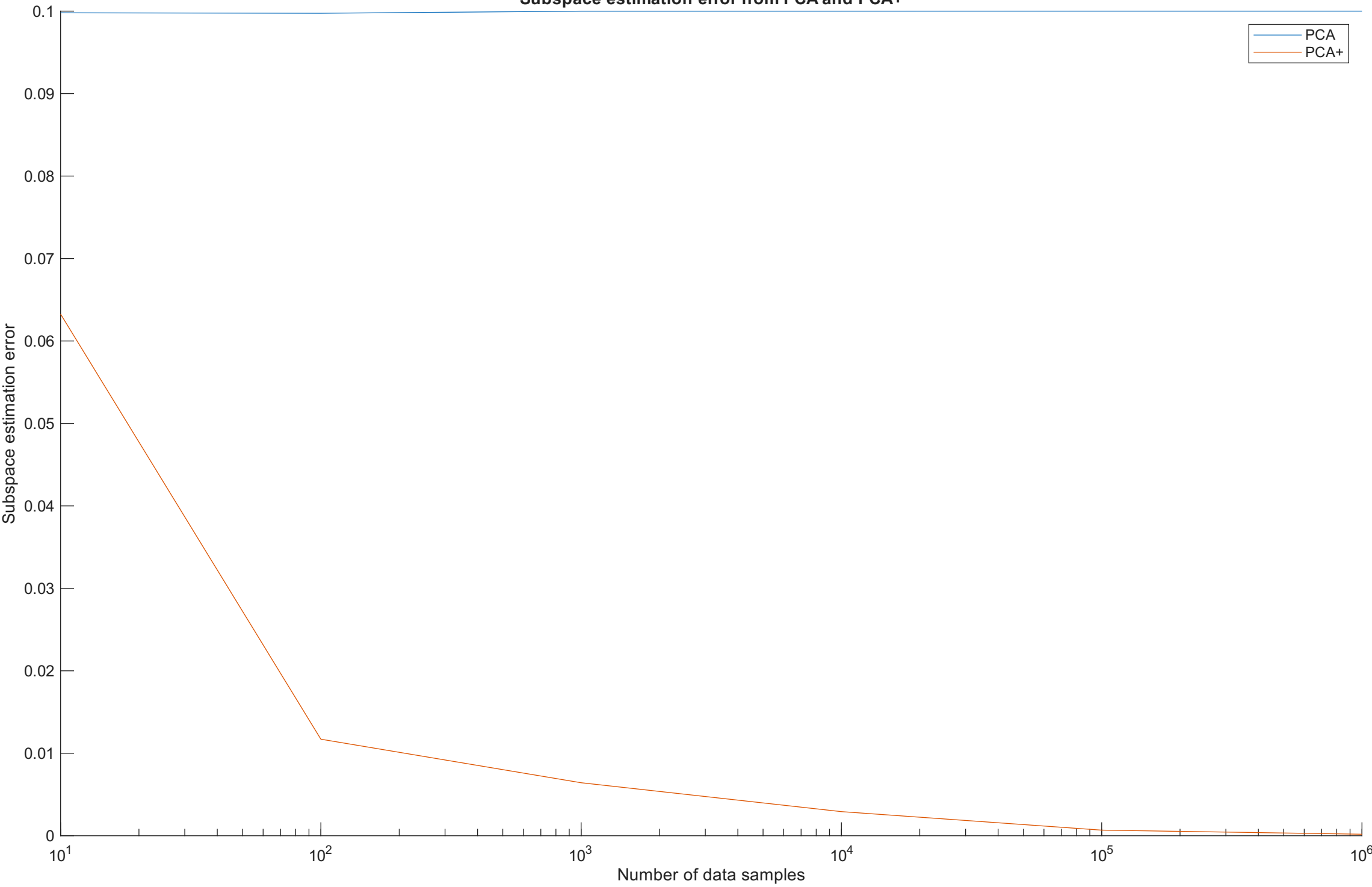
Subspace estimation error from PCA and PCA+
